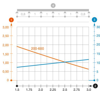
Load diagram, cable ladder, type LG 45 NS
